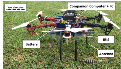
Figure 3: ASTRO hexadrone
